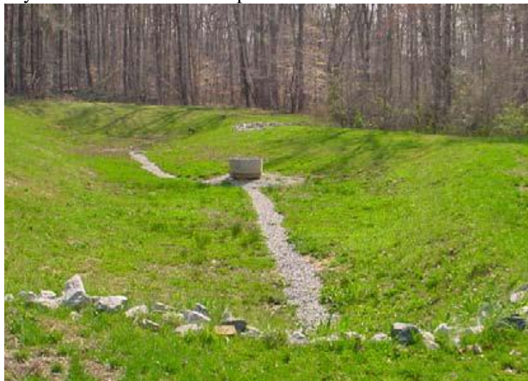
Figure 2-14 Dry detention basin
