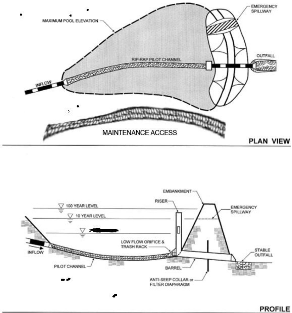
Figure 2-15 Dry detention basin schematic
