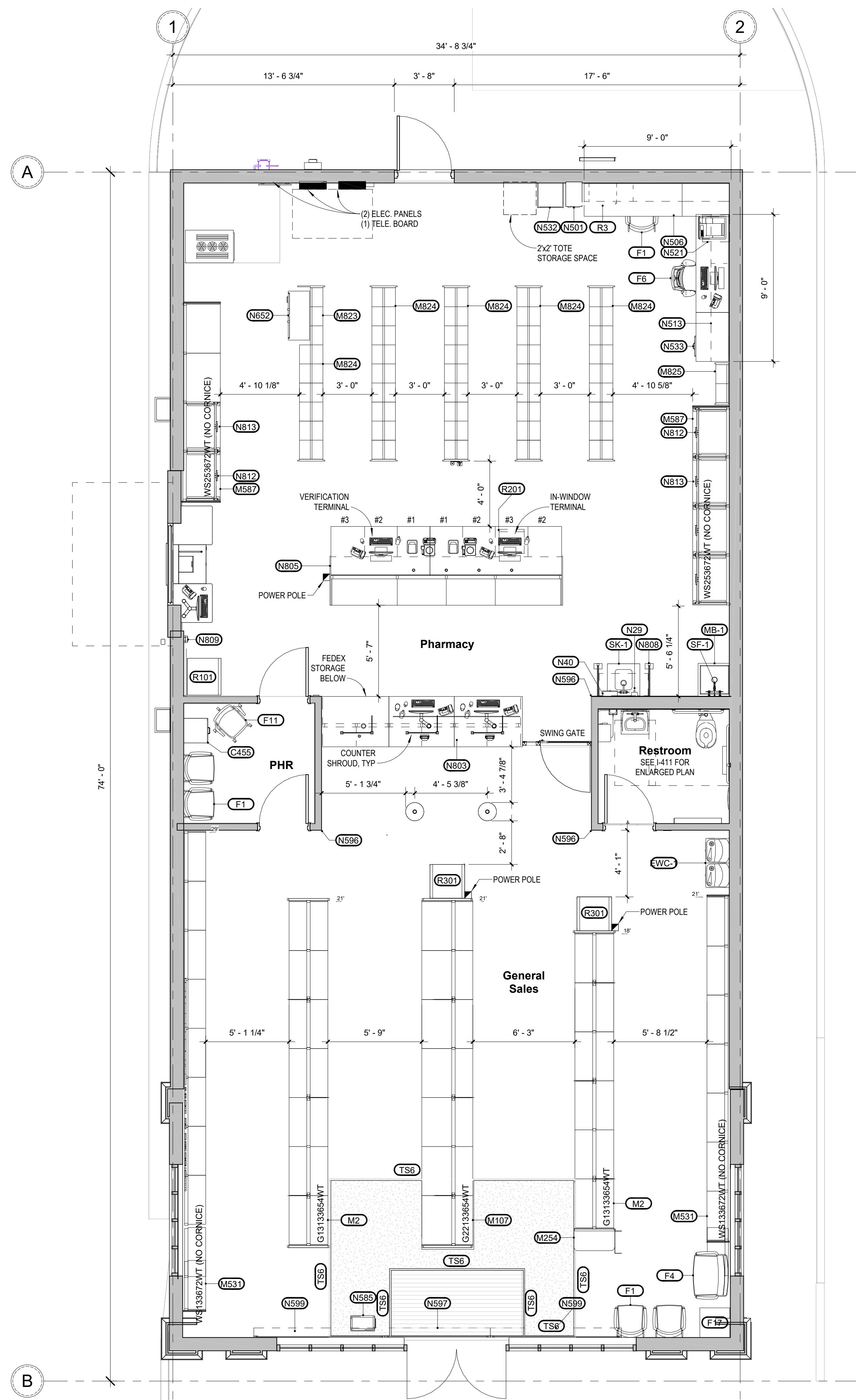
1 Fixture Floor Plan 1/4" = 1'-0"
