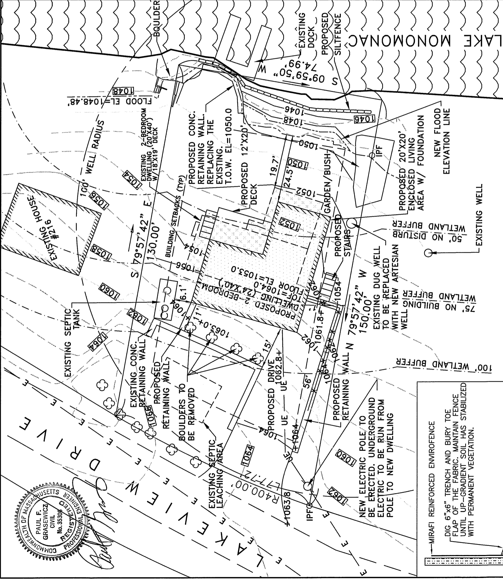
PLAN 1"=20'
